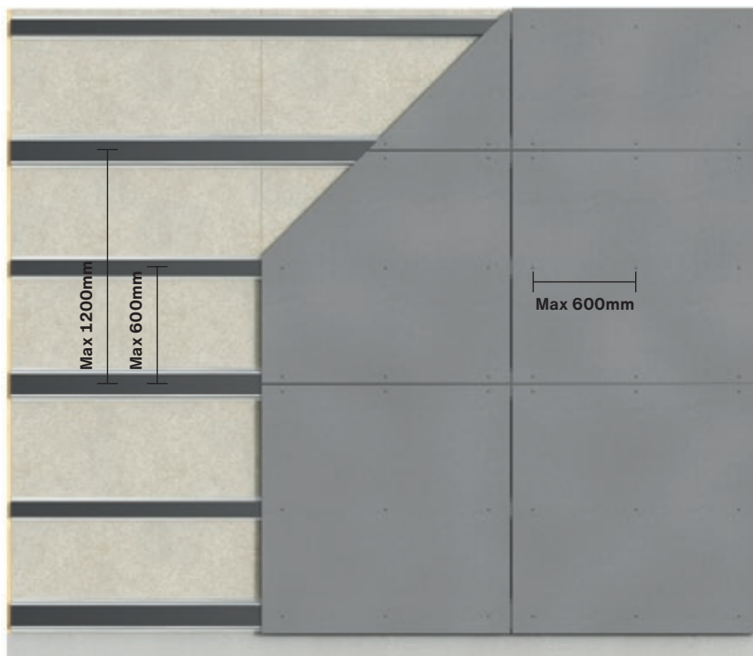
Swisspearl facade boards installed on horizontal VFL profiles
