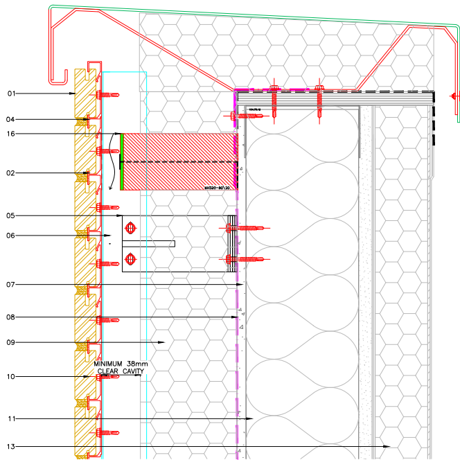
Coping Detail
